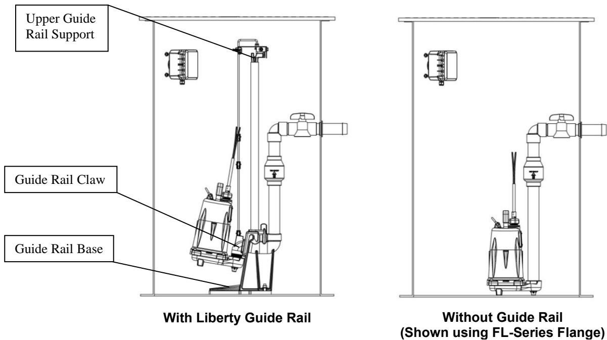
Fig. A – Typical Pump Installation
