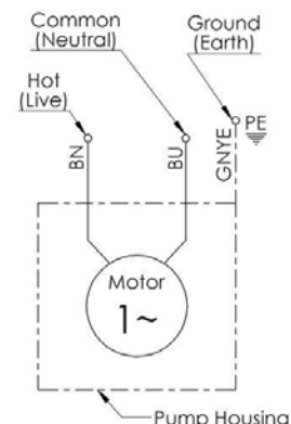
Fig. C – Direct Wiring of 230V 1-Phase Pumps
