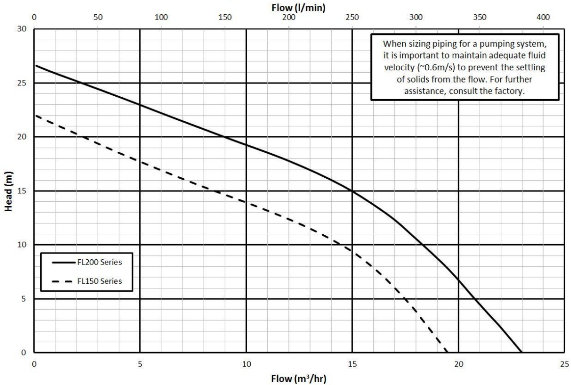
Fig. E – Hydraulic Performance Curves
