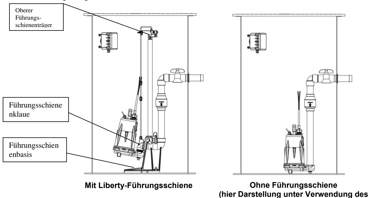
Abb. A – Standard-Pumpeninstallation
